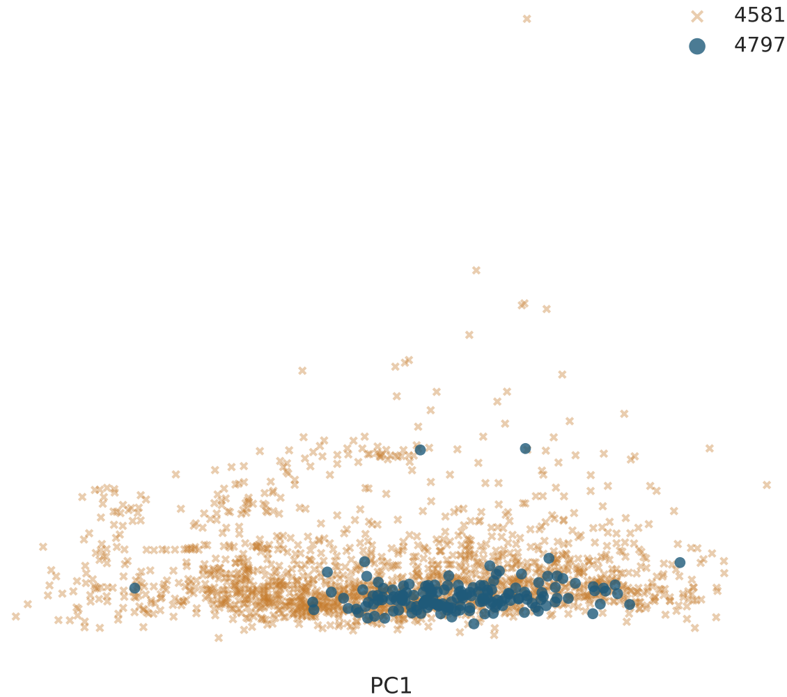
PCA colored by source project
